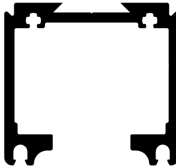
200A Top Track 45mm x 42mm
