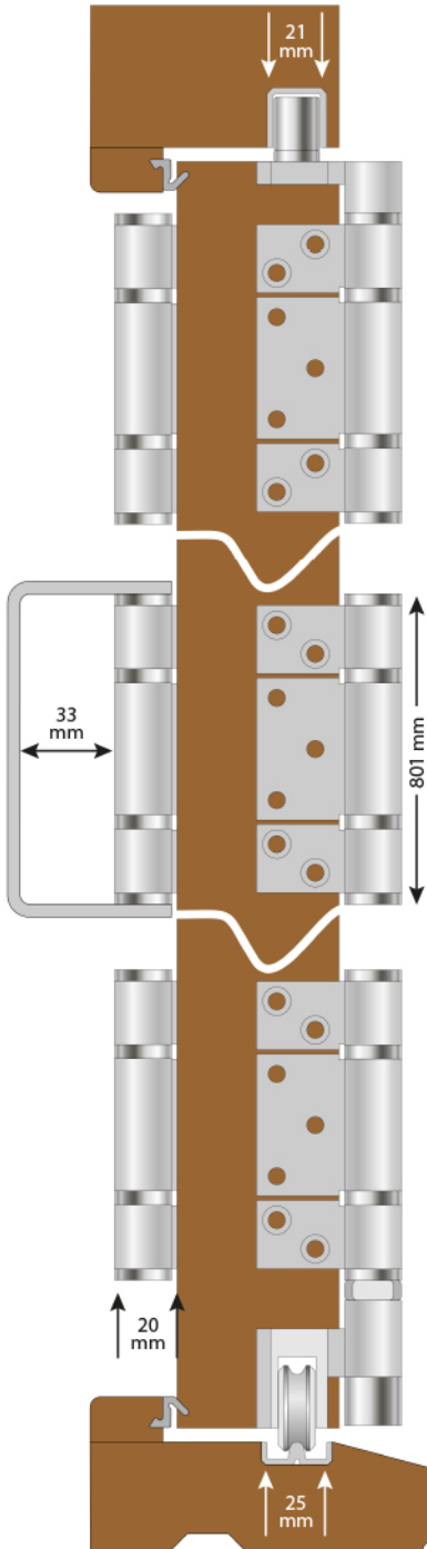
End elevation with recessed track option
