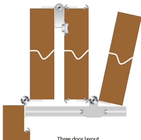
Three door layout
